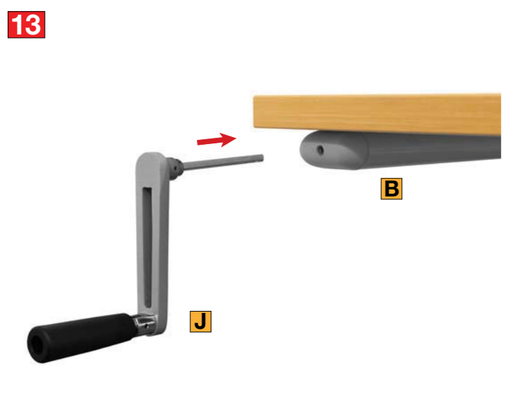
13. To fix the handle into position, take Handle 'J' and insert the pin into the opening on the end of component 'A' or 'B', as above.
